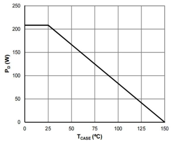
Figure 10: Power De-rating
